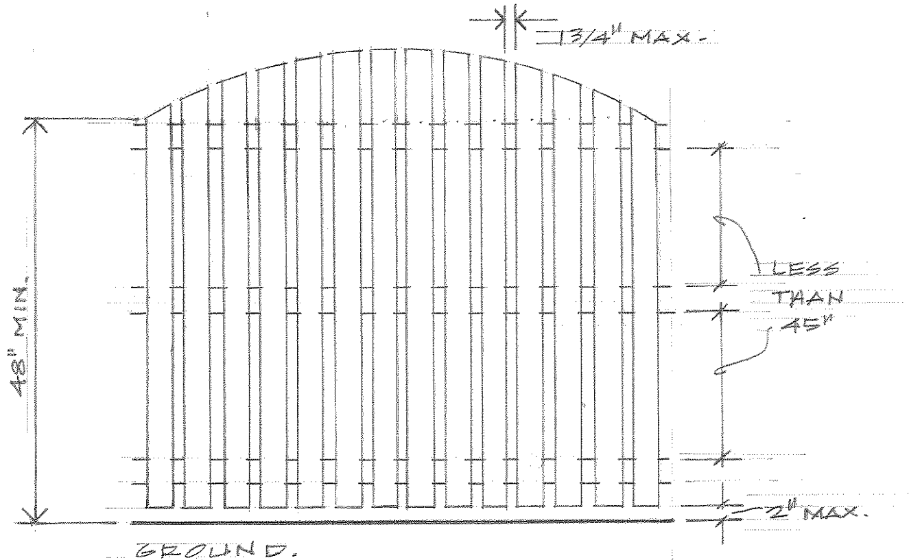
4. PICKETS W/ HORIZONTAL LESS THAN 45"
