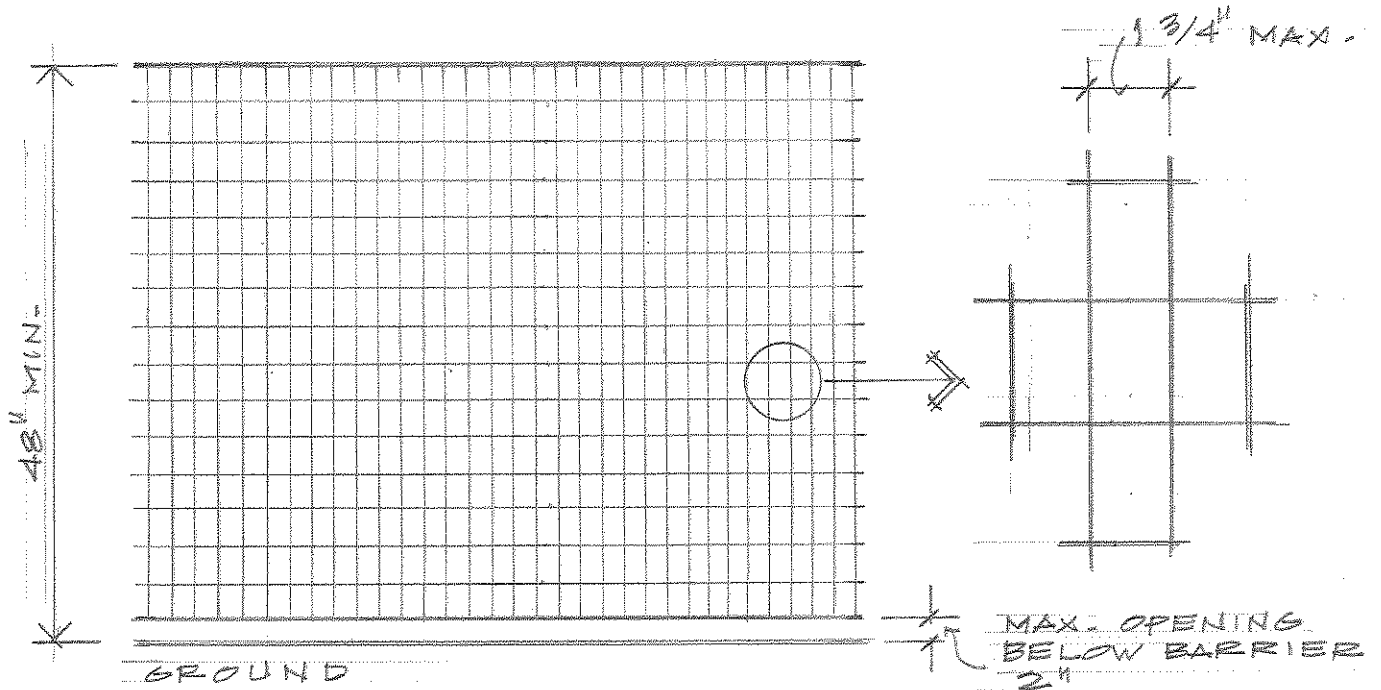
3. WIRE MESH
